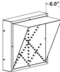
DVS-4 Sun Visor
